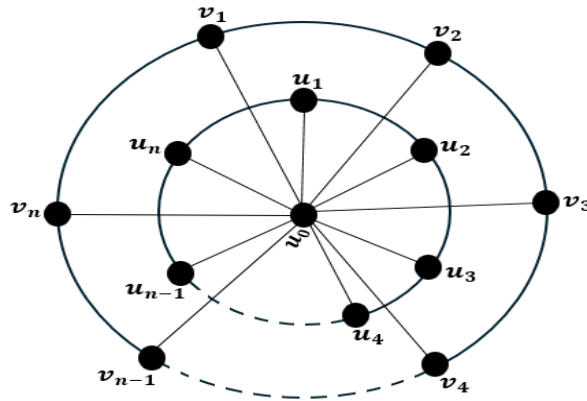
FIGURE 2. An LD labeling for the double wheel graph W_{n,n} for n is even and n \geq 4 .
