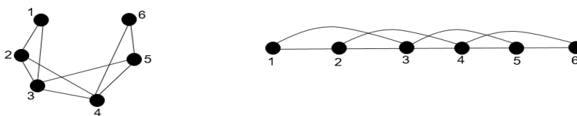
FIGURE 9. An LD labeling for P_6^2 and P_6(2) .
