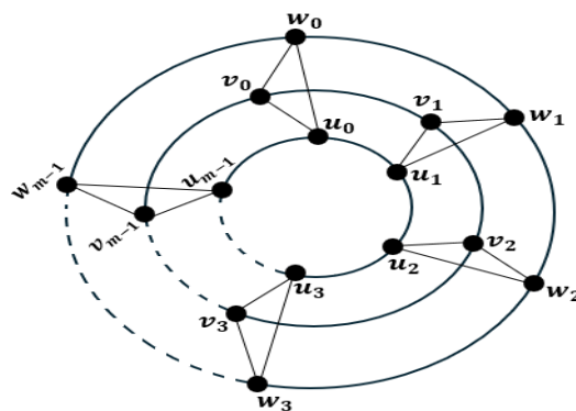
FIGURE 4. An LD labeling for the graph C_3 \times C_m , m is even and m \geq 3 .
