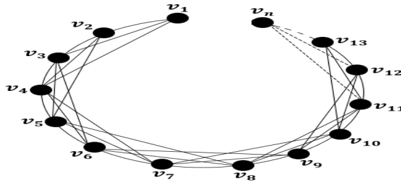
FIGURE 10. An LD labeling for the graph P_n^3 , when n \equiv 0 \pmod{6} .
