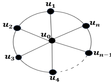
FIGURE 1. An LD labeling for the wheel graph W_n , for all n > 1 .
