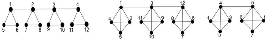
FIGURE 6. LD labeling graphs.
