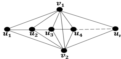
FIGURE 7. An LD labeling for the double fan graph for all n \geq 3 .
