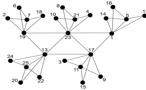
FIGURE 5. An LD labeling for the graph TS'_3 \odot S_4 .
